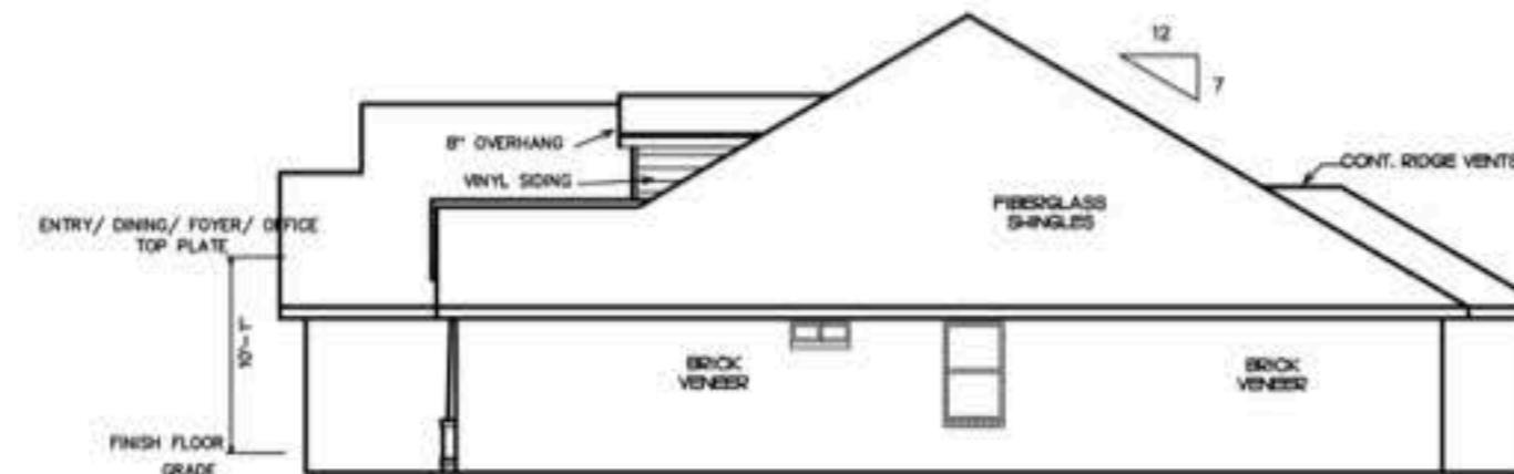
RIGHT ELEVATION SCALE 1/8" = 1'-0"
